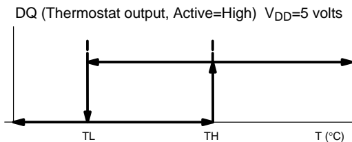
THERMOSTAT OUTPUT OPERATION Figure 3
