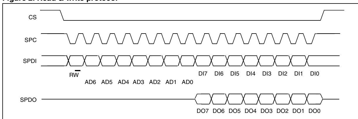
Figure 2. Read & write protocol
