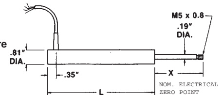
Model JEC Free Unguided
