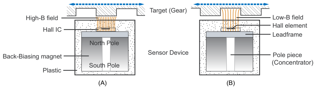
Figure 2. Device Cross Section. Motion of the target is detected by the Hall element mounted on the Hall IC. Panel A, the presence of a tooth feature on the target is distinguished by a high magnetic flux density, B. Panel B, the presence of a valley feature is distinguished by its low magnetic flux density.
