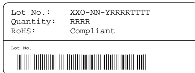
Figure 18: First label on reel: XX = Sensor Type (21 for SHT21), O = Output mode (D = Digital, P = PWM, S = SDM), NN = Chip Version, Y = last digit of year, RRRR = number of sensors on reel, TTTT = Traceability Code.
