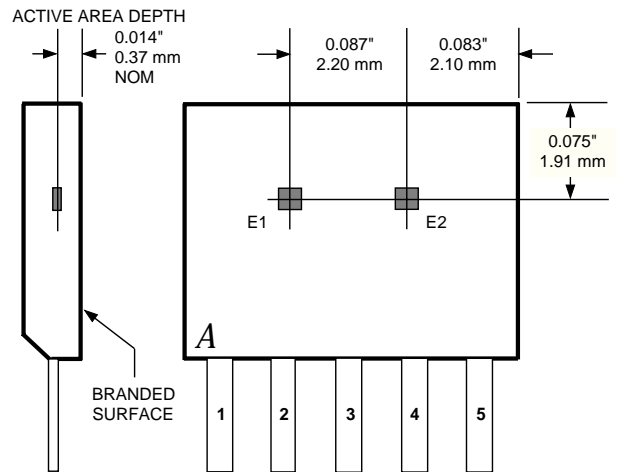
Figure 5 SENSOR LOCATIONS (±0.005" [0.13 mm] die placement)
