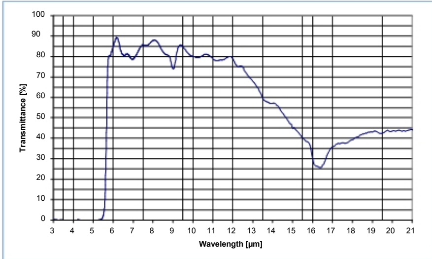
Figure 3 Transmission Curve for Excelitas Standard Filter
