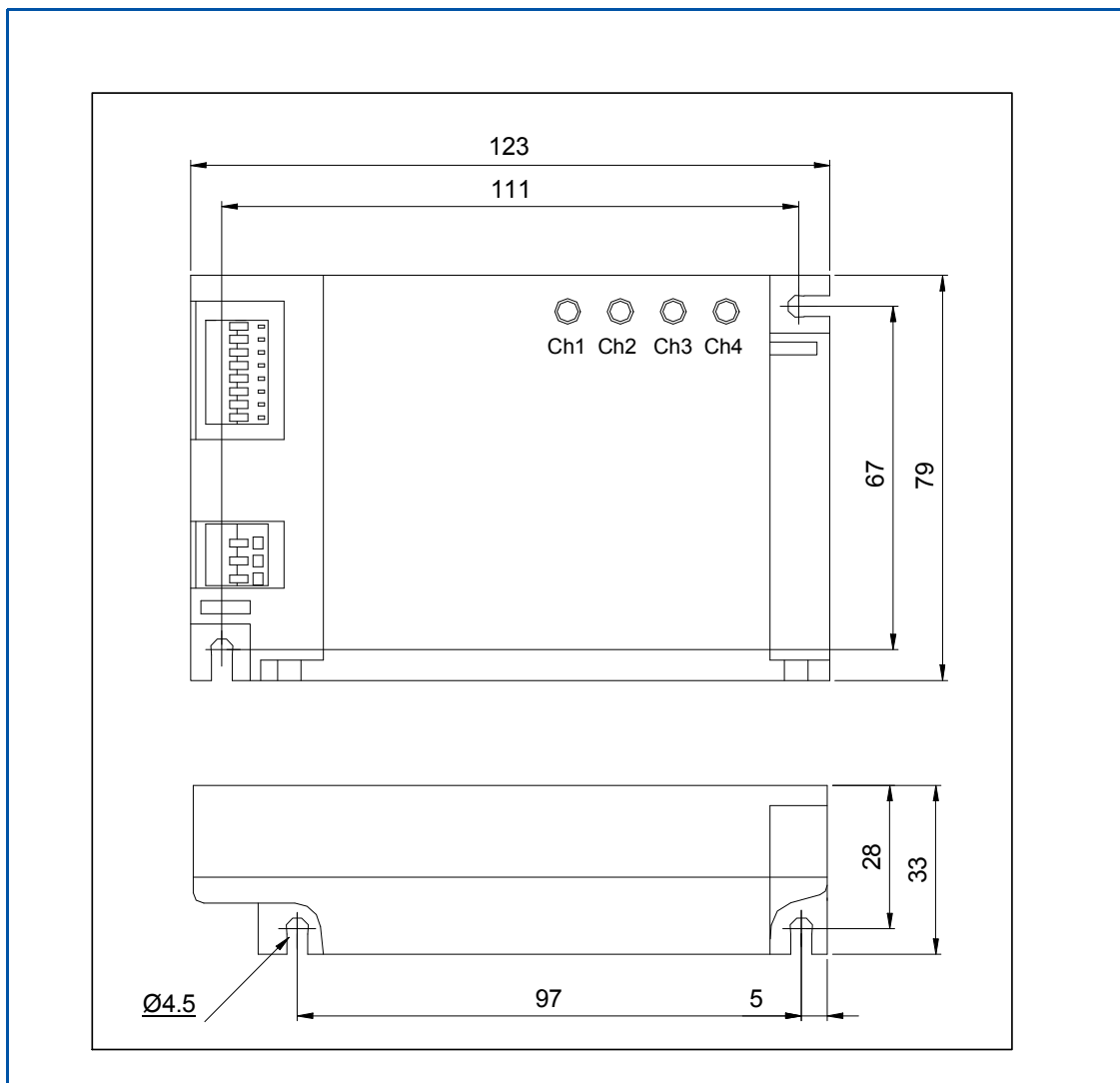
Figure 1 Dimensions of the power supply unit
