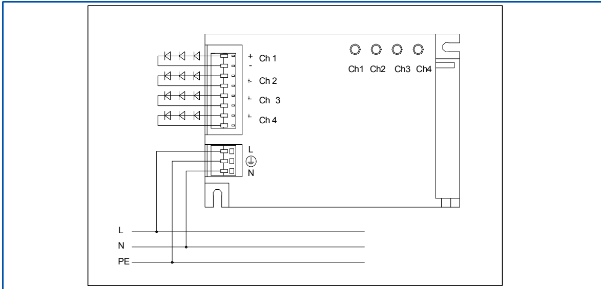
Figure 2 Schematic diagram of the power supply unit
