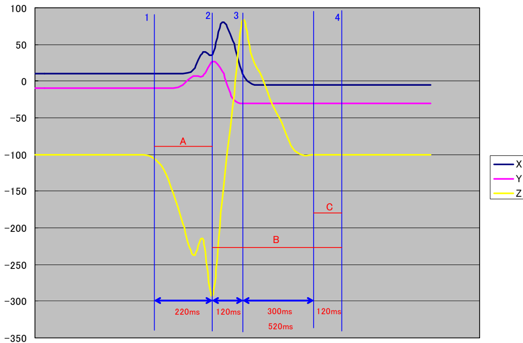
Figure 5 Move to Z-axis (plus) direction
