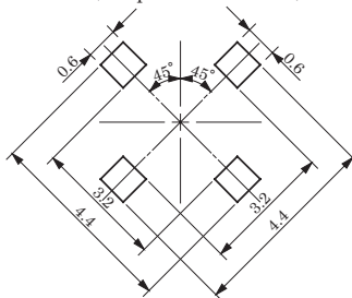
Recommended footprint (component-side view)
