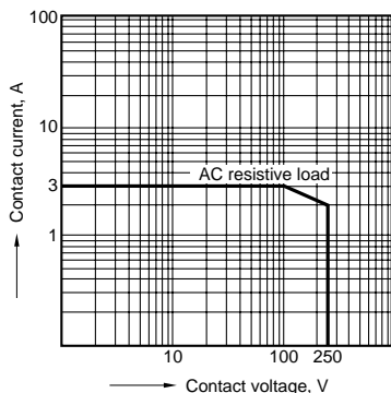
1-(1). Maximum value for switching capacity (Standard type)
