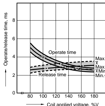
2. Operate/release time
