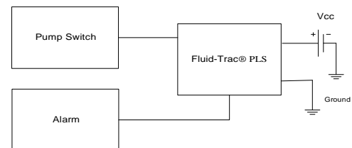
Figure1. Fluid-Trac® PLS Fill and Alarm
