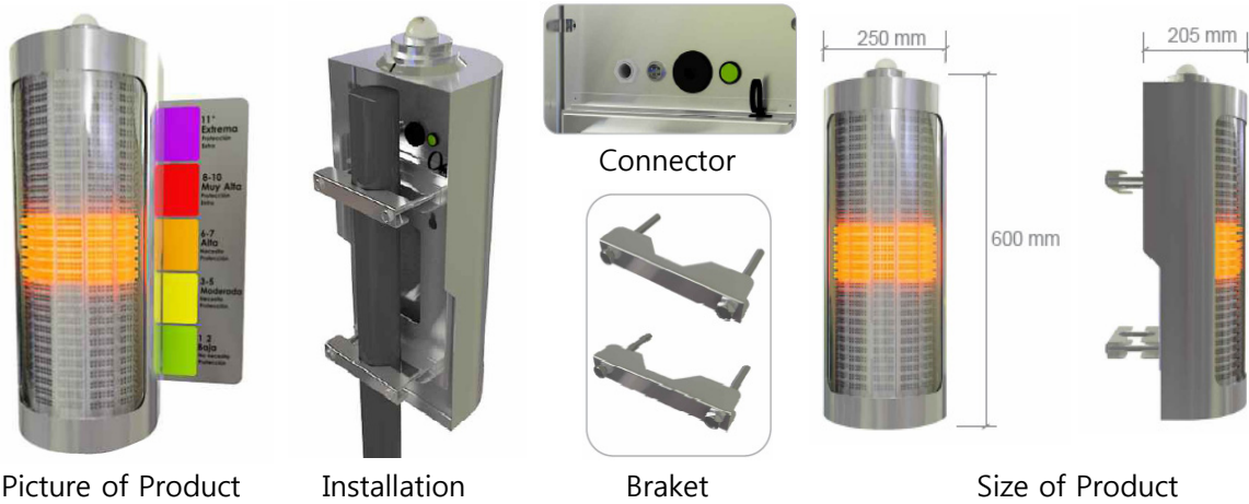
Fig1. Physical Dimentions
