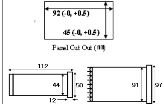
Fig. 2 Size of UV Radiometer 5.0
