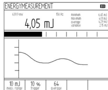
display for energy measurement
