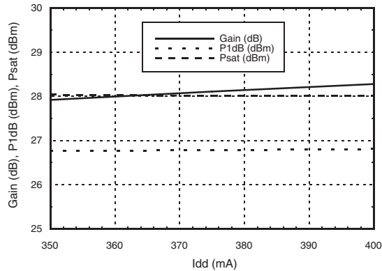
Gain & Power vs. Supply Current @ 27 GHz
