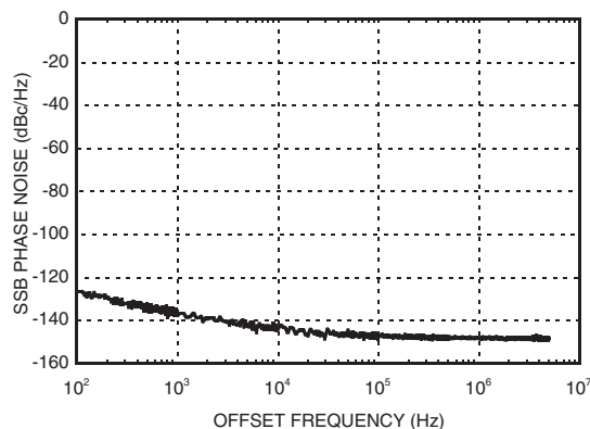
SSB Phase Noise Performance @ F_{in} = 3\text{ GHz} P_{in} = 0\text{ dBm} , T = 25\text{ }^{\circ}\text{C}
