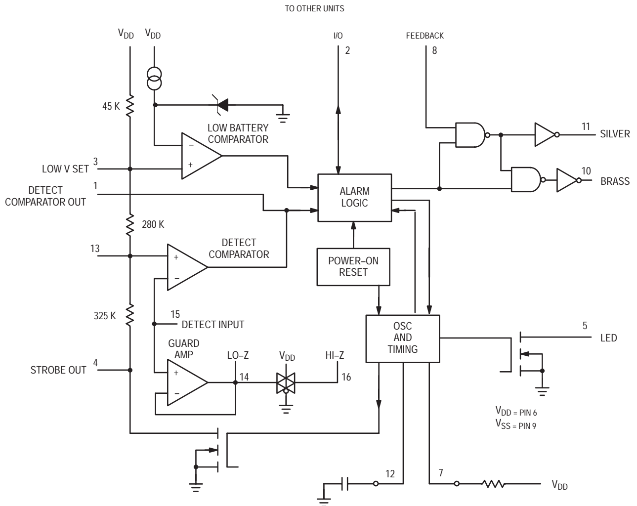
Figure 1. Block Diagram
