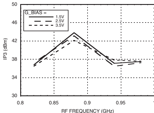
IP3 vs G_BIAS, LO = 1060 MHz [2]
