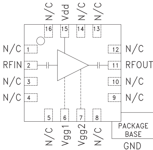
TOP VIEW Vgg1, Vgg2: Optional Gate Bias
