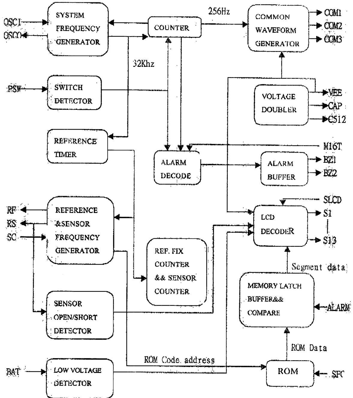
BLOCK DIAGRAM :
