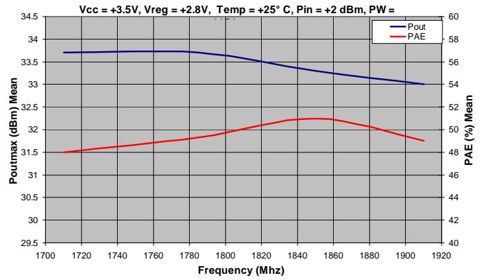
DCS/PCS Maximum Output Power and PAE
