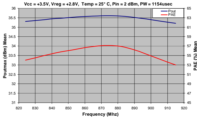
GSM850/GSM900 Maximum Output Power and PAE
