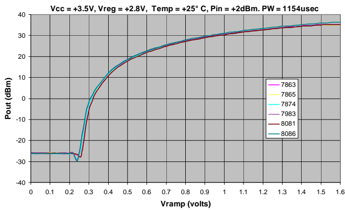
GSM (902.4MHz) Pout vs Vramp
