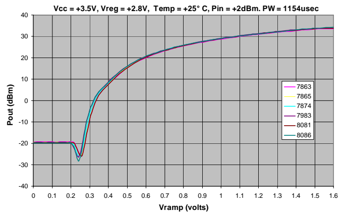
DCS (1747.4 MHz) Pout vs Vramp
