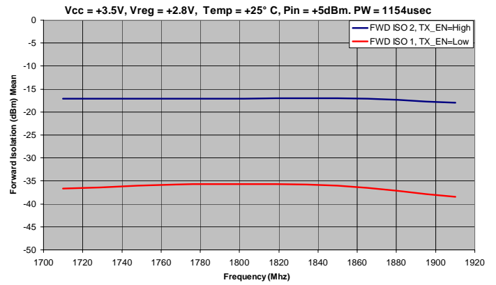
DCS/PCS Forward Isolation
