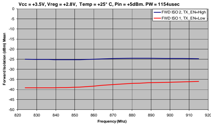
GSM850/GSM900 Forward Isolation
