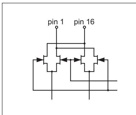
Figure 18: Equivalent Circuits
