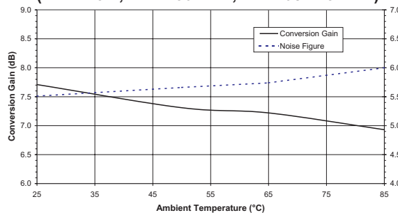
Figure 6: Typical Conversion Gain and Noise Figure vs. Ambient Temperature ( V_{DD} = +5\text{ V} , f_{RF} = 450\text{ MHz} , f_{IF} = 1087.75\text{ MHz} )
