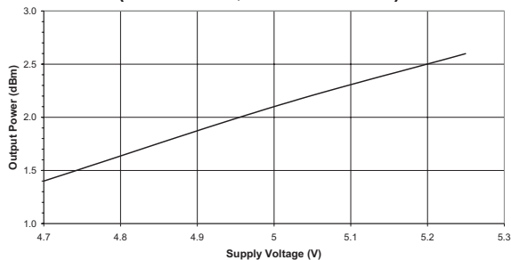
Figure 10: Typical Local Oscillator Output Power vs. Supply Voltage ( T_A = +25\text{ }^{\circ}\text{C} , f_{LO} = 1500\text{ MHz} )
