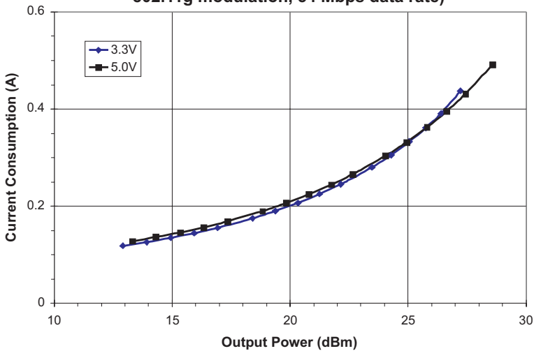
Figure 4: Typical Current vs. Output Power (T A = +25 °C, V REF1 = V REF2 = +2.85 V 802.11g modulation, 54 Mbps data rate)
