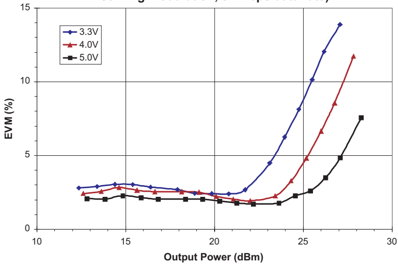
Figure 3: Typical EVM (1) vs. Output Power (T A = +25 °C, V REF1 = V REF2 = +2.85 V 802.11g modulation, 54 Mbps data rate)
