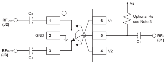
Figure 1: Pinout Diagram
