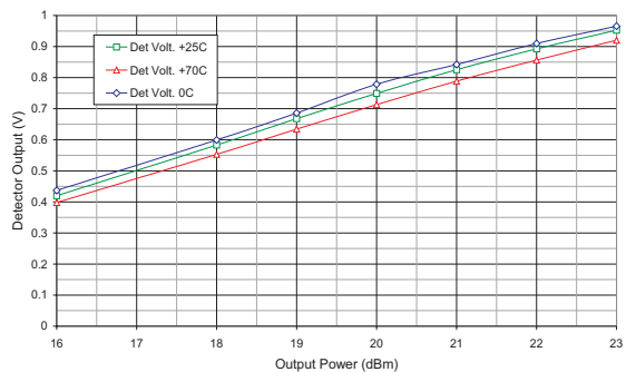
Figure 13: Power Detector Voltage vs. Output Power at 2.462 GHz, 3.3 V (IEEE 802.11b @ 11 Mbps)
