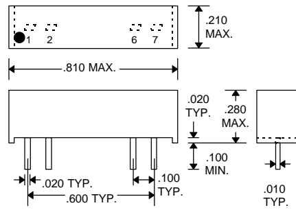
Package Dimensions
