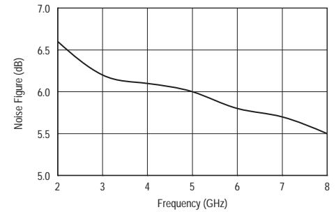
Noise Figure (+11 V, 50 mA)
