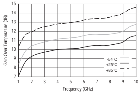
Gain Over Temperature (+11 V, 50 mA)
