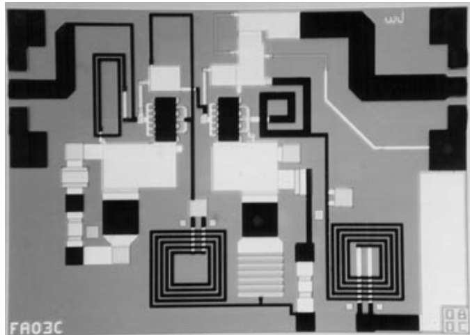
ICA1007 Chip Outline
