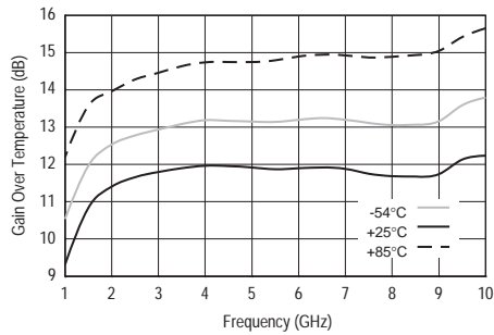
Gain Over Temperature (+11 V, 80 mA)
