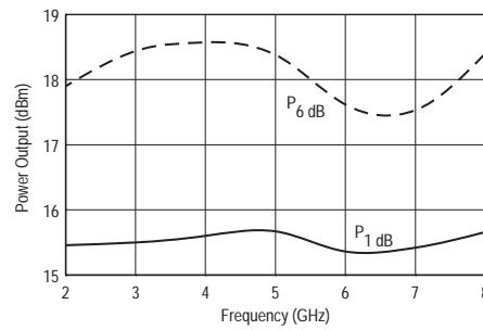
Power Output (+11 V, 50 mA)
