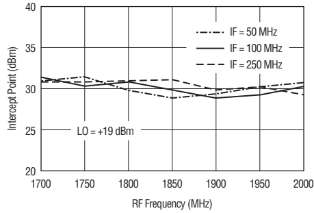
3IIP vs. RF Frequency
