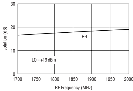
R-I Isolation vs. RF Frequency
