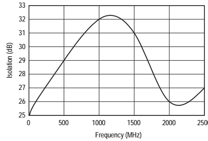
R-I Isolation vs. Frequency
