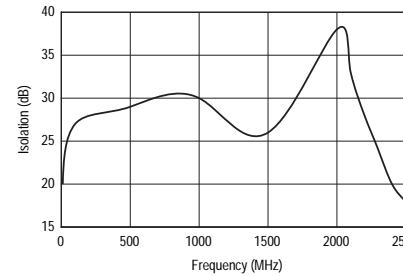
R-I Isolation vs. Frequency
