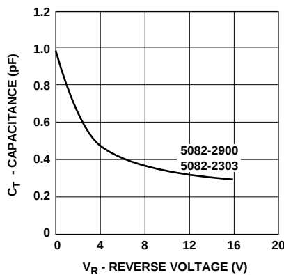
Figure 4. 5082-2300 and 5082-2900 Series Typical Capacitance vs. Reverse Voltage.
