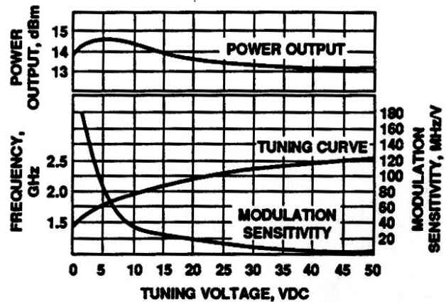
Figure 4. VTO-S150 Power Output, Frequency and Modulation Sensitivity vs. Tuning Voltage.
