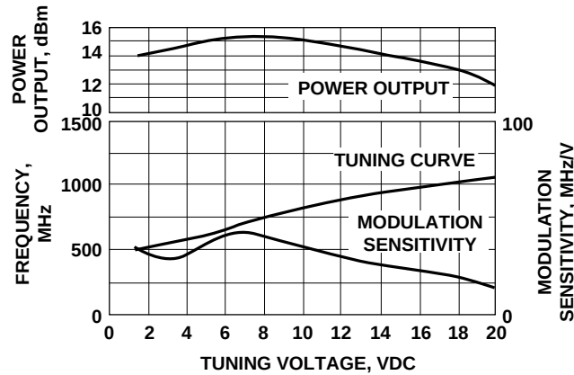
Figure 3. VTO-9050 Power Output, Frequency and Modulation Sensitivity vs. Tuning Voltage.
