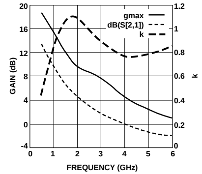
Figure 8. Gain vs. Frequency at 2.7 V, 2 mA.
