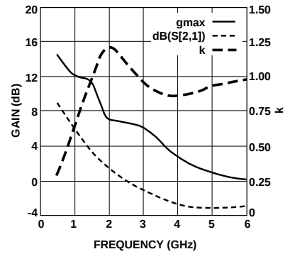
Figure 7. Gain vs. Frequency at 1 V, 1 mA.
