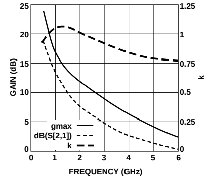
Figure 13. Gain vs. Frequency at 5 V, 10 mA.
