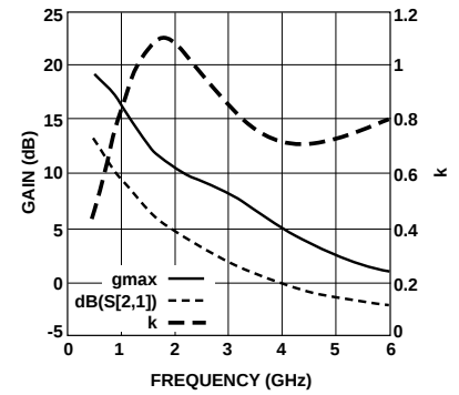
Figure 11. Gain vs. Frequency at 5 V, 2 mA.
