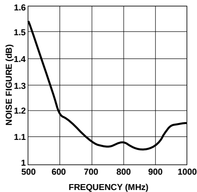
Figure 18. Noise Figure vs Frequency.
