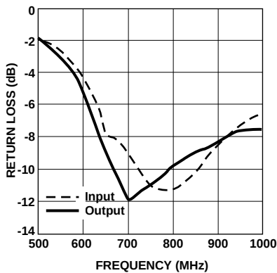
Figure 19. Input/Output Return Loss.
