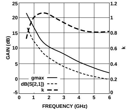
Figure 9. Gain vs. Frequency at 2.7 V, 5 mA.
