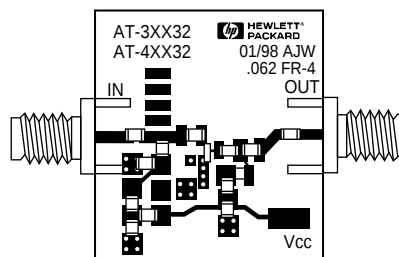
Figure 16. 1X Artwork showing Component Placement.
