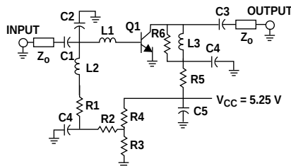
Figure 14. Schematic Diagram.
