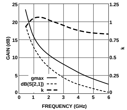
Figure 10. Gain vs. Frequency at 2.7 V, 10 mA.
