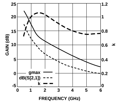
Figure 12. Gain vs. Frequency at 5 V, 5 mA.
