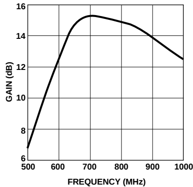
Figure 17. Gain vs Frequency.
