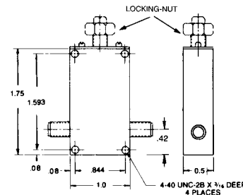
Figure 1 AV-18265 and AV-26540
