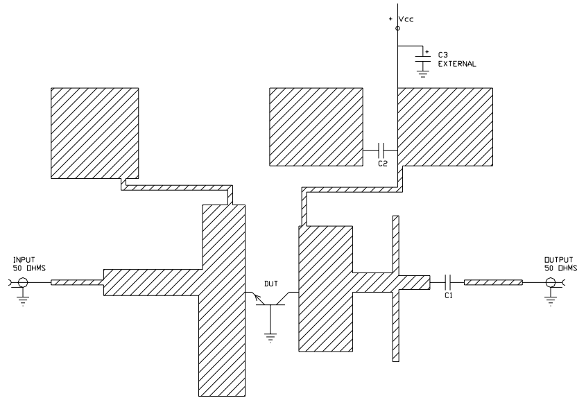
ELECTRICAL SCHEMATIC
