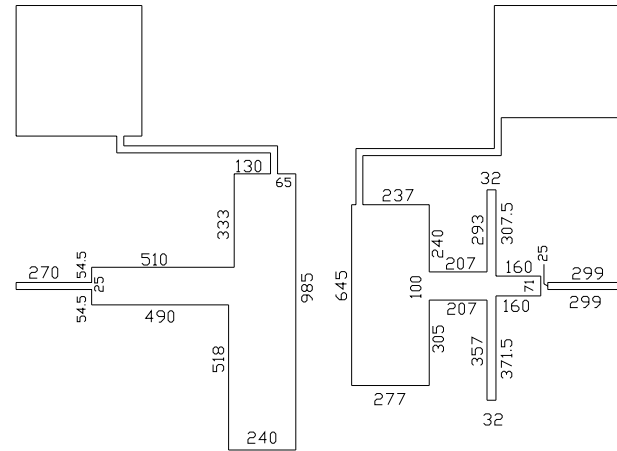
CIRCUIT DIMENSIONS IN MILS
