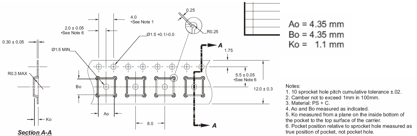
Figure 12. Tape and Reel Drawing
