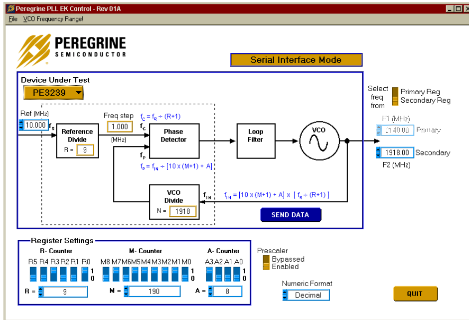
Figure 4. PE3239 Software Control Panel
