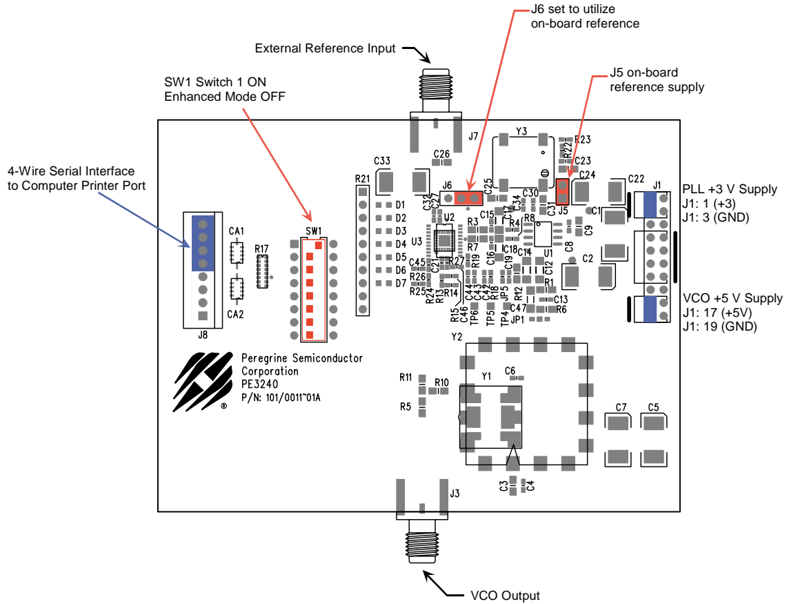
Figure 2. Evaluation Kit Default Jumper & Switch Settings.
