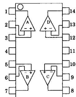
NJM12902D1/12902M NJM12902E/12902V
