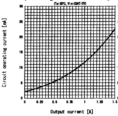
NJM2396F05 Circuit operating current vs. Output current
