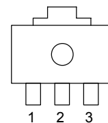
NJM1431AU
