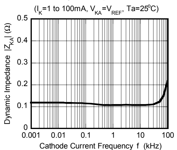
Dynamic Impedance
