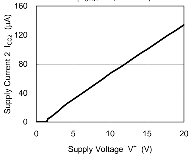
Supply Current 2 vs. Supply Voltage ( V_{STBY}=0V, T_a=25^\circ C )
