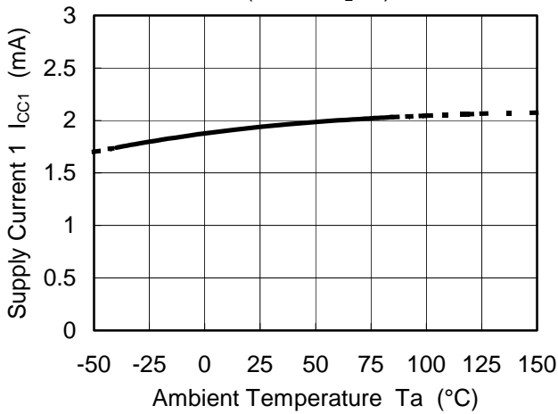
Supply Current 1 vs. Temperature ( V^+=5V, R_L=\infty )
