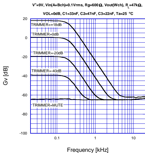
fig.25 LPF Characteristics (C1)
