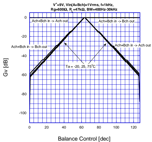
fig.6 Voltage Gain vs Balance Control
