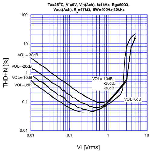
fig.10 THD+N vs Input Voltage (Ach, Bch)
