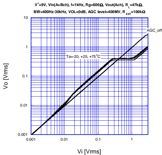
fig.16 AGC Characteristics ( T_a )
