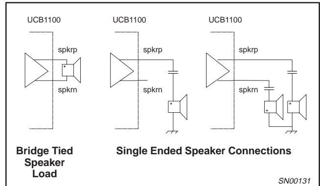
Figure 6. Possible Speaker Connections
