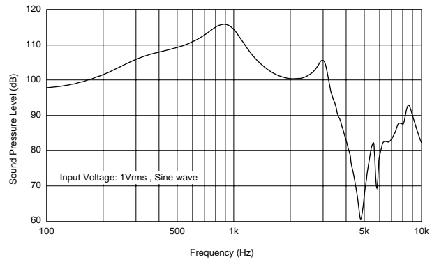
Frequency Response
