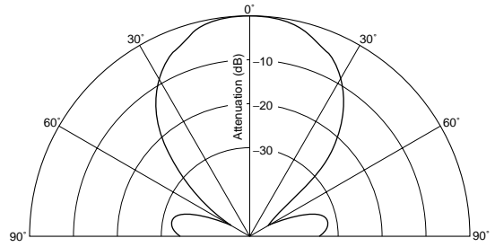
Directivity in sensitivity
