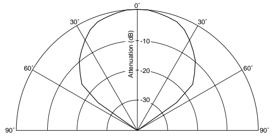
Directivity in overall sensitivity
