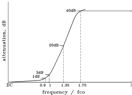
LOW PASS TYPICAL FREQUENCY RESPONSE
