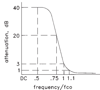
HIGH PASS TYPICAL FREQUENCY RESPONSE
