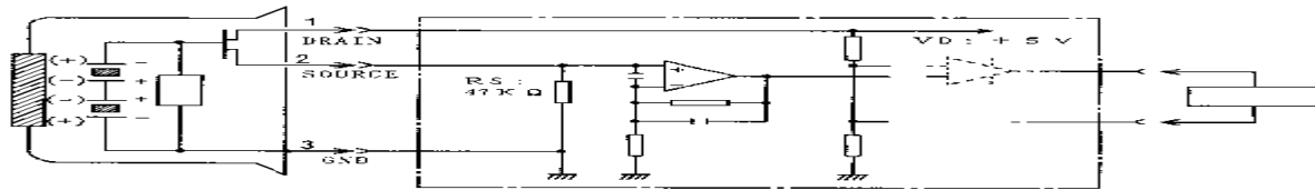
TEST SET-UP BLOCK DIAGRAM (FIGURE 3)
