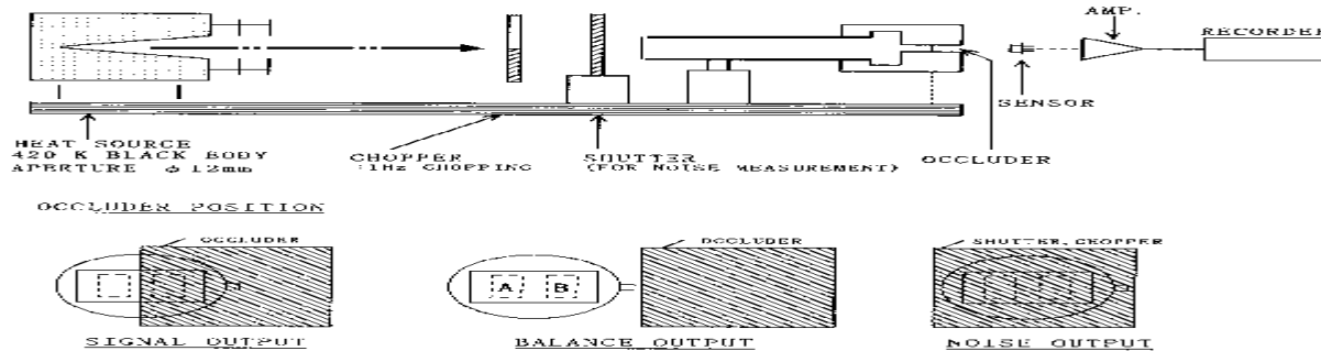
TEST SET-UP BLOCK DIAGRAM (FIGURE 3)
